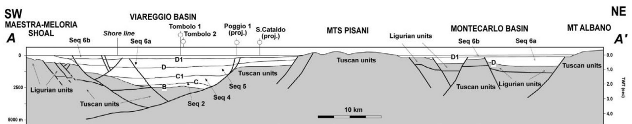
Fig. 7 - SW-NE geological section (time and depth) of the Meloria-Maestra Shoal-Viareggio Basin-Mts Pisani-Montecarlo Basin-Mt Alabano area derived from seismic data and the well Poggio 1 (location in Figure 3). Time velocity is derived from well Tombolo 1.
